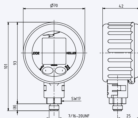
LEO2 with rubber cover
